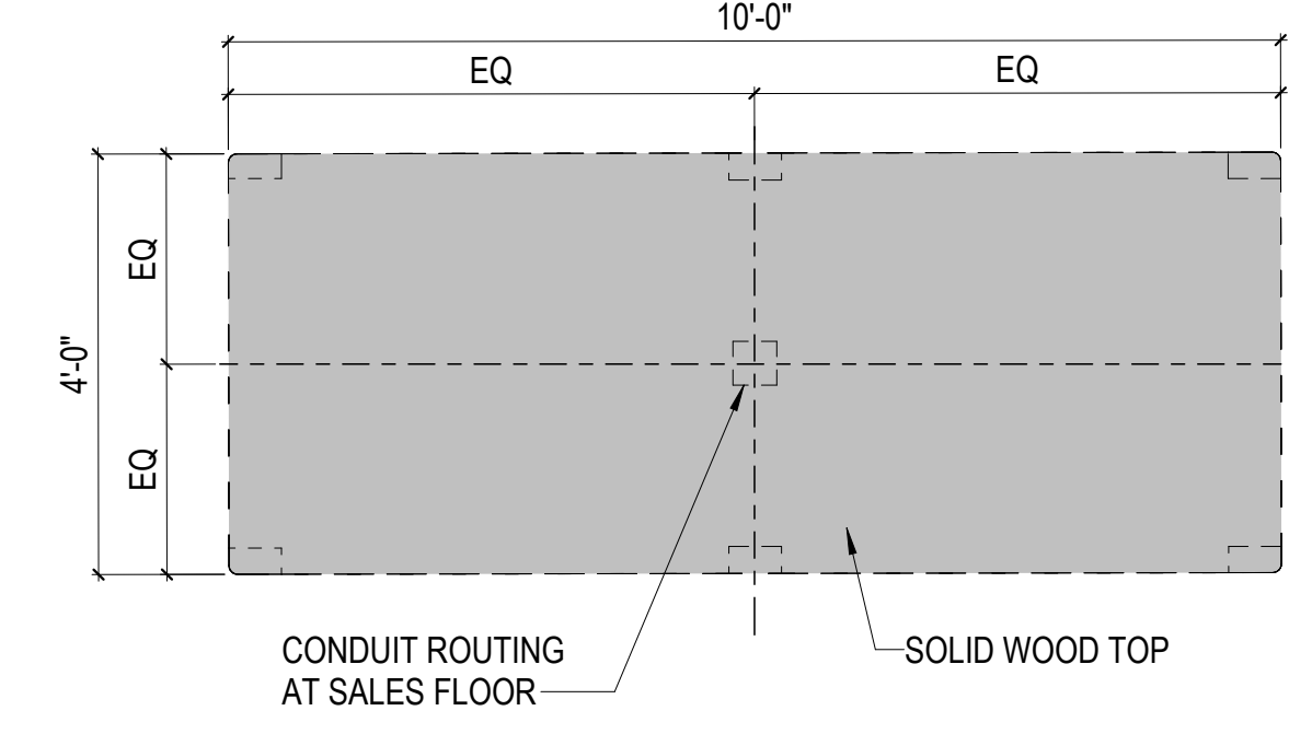
2 DESIGN LAB TABLE- OVERALL ENLARGED PLAN 1/2" = 1'-0"
